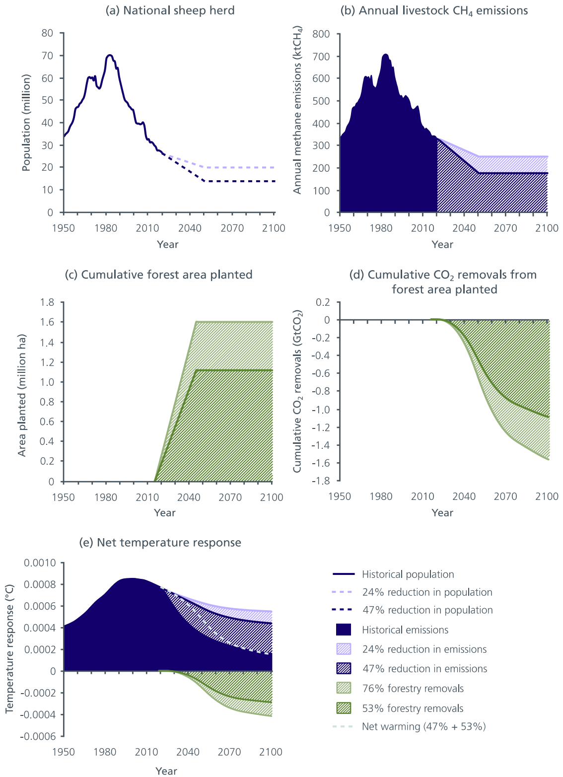
Figure A2.3: Illustrative scenarios for offsetting warming from livestock methane emissions for the national sheep herd using GWP*.
