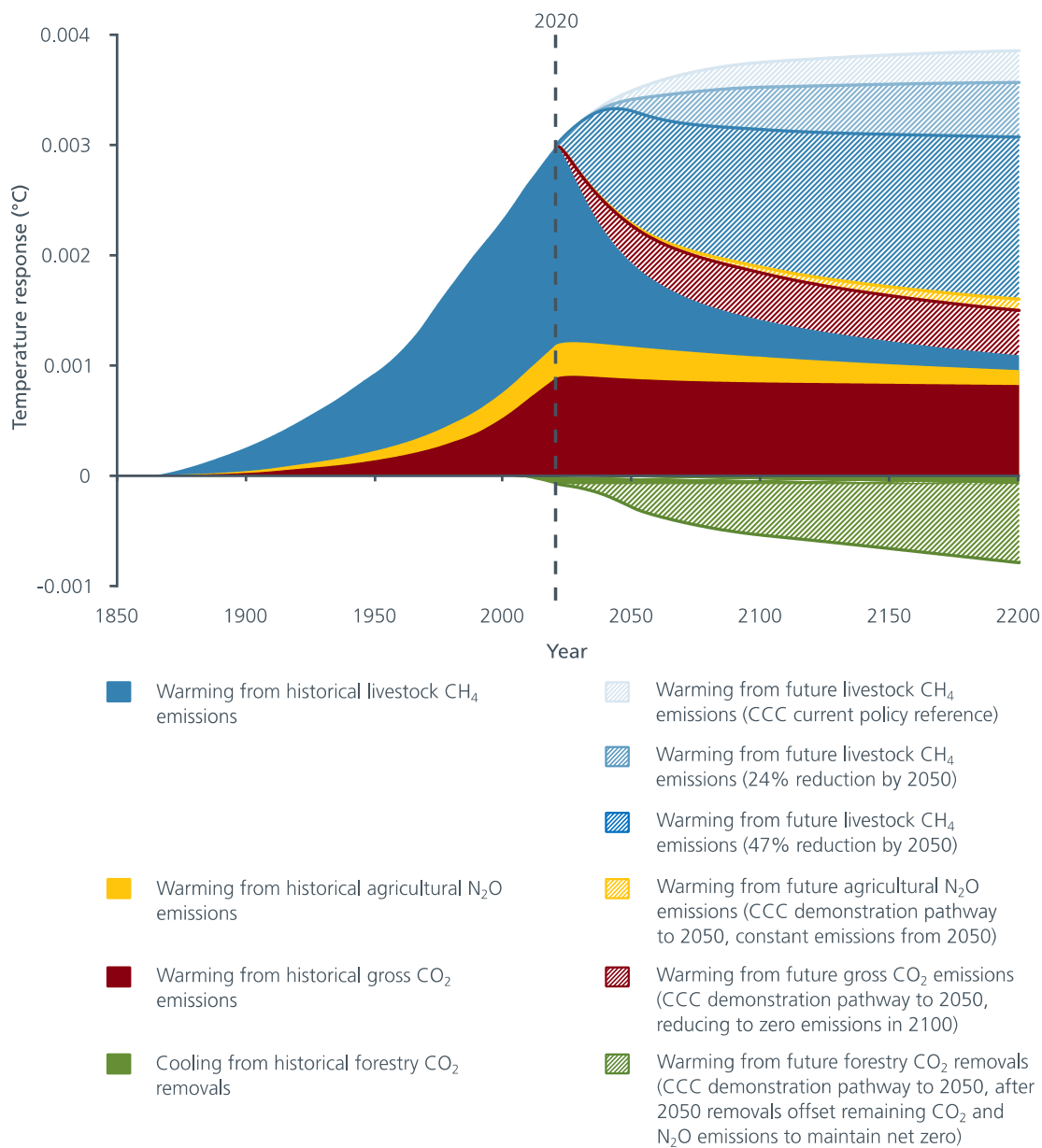
Figure 10: Warming from past emissions and illustrative pathways for future emissions. The solid shaded areas show the warming from past emissions – this warming is already ‘locked in’. The hatched areas show the warming from future emissions that can potentially be avoided by reducing emissions. Deep, rapid and sustained reductions in gross emissions of livestock methane, fossil carbon dioxide and agricultural nitrous oxide will be needed – as well as enhanced carbon dioxide removals from forests – to minimise the warming from New Zealand’s future emissions. The temperature response from emissions and removals from forestry prior to 1990 is not shown. The temperature responses were calculated by stacking the temperature responses for one-off emissions and removals from Figure 1.
